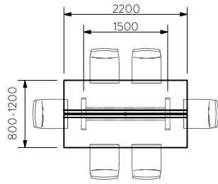
CABLE TRAY 1500/1420
