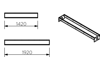
SUPPORT BEAMS
